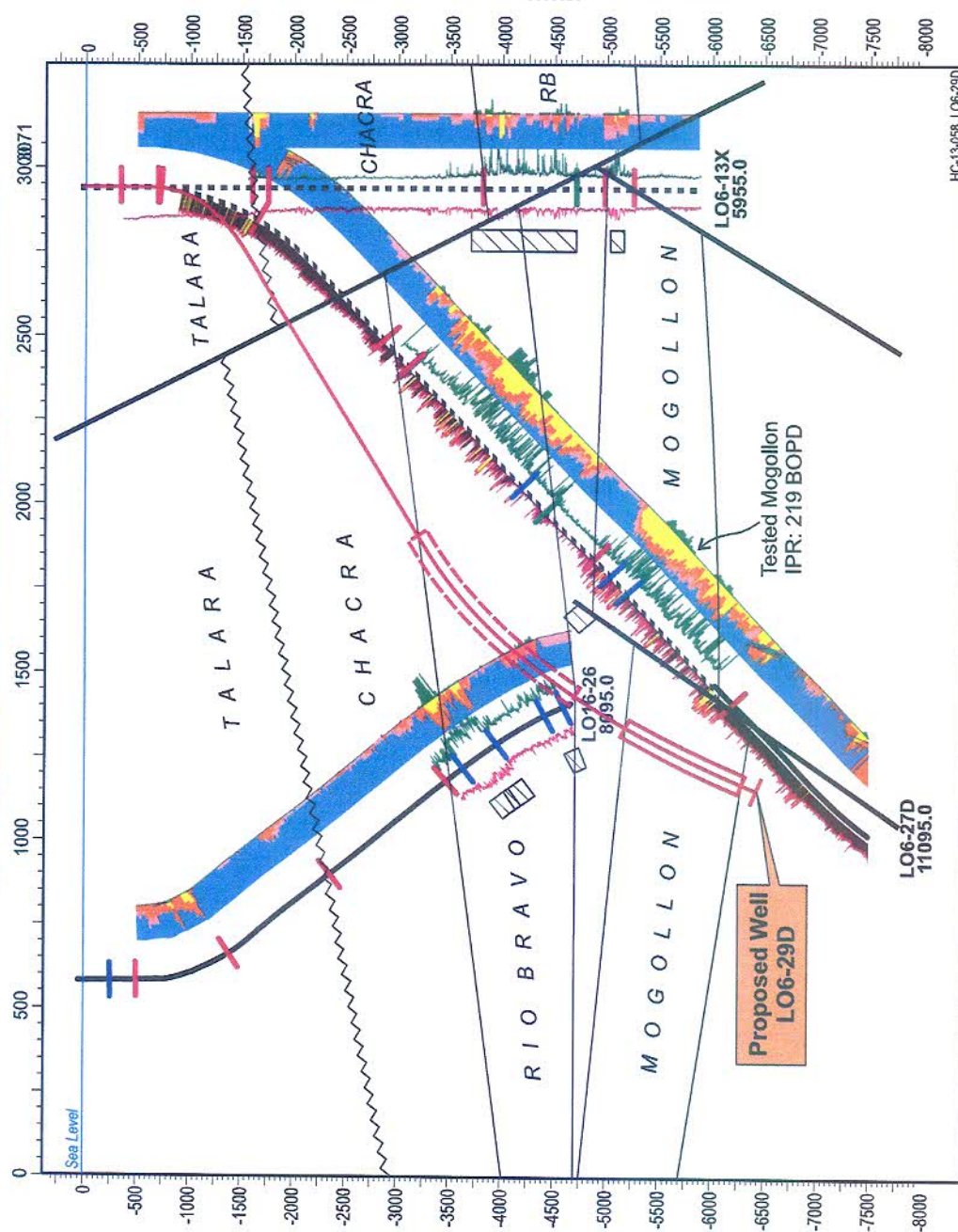
Fig. 3 SW-NE Structural Section for proposed well LO6-29D
