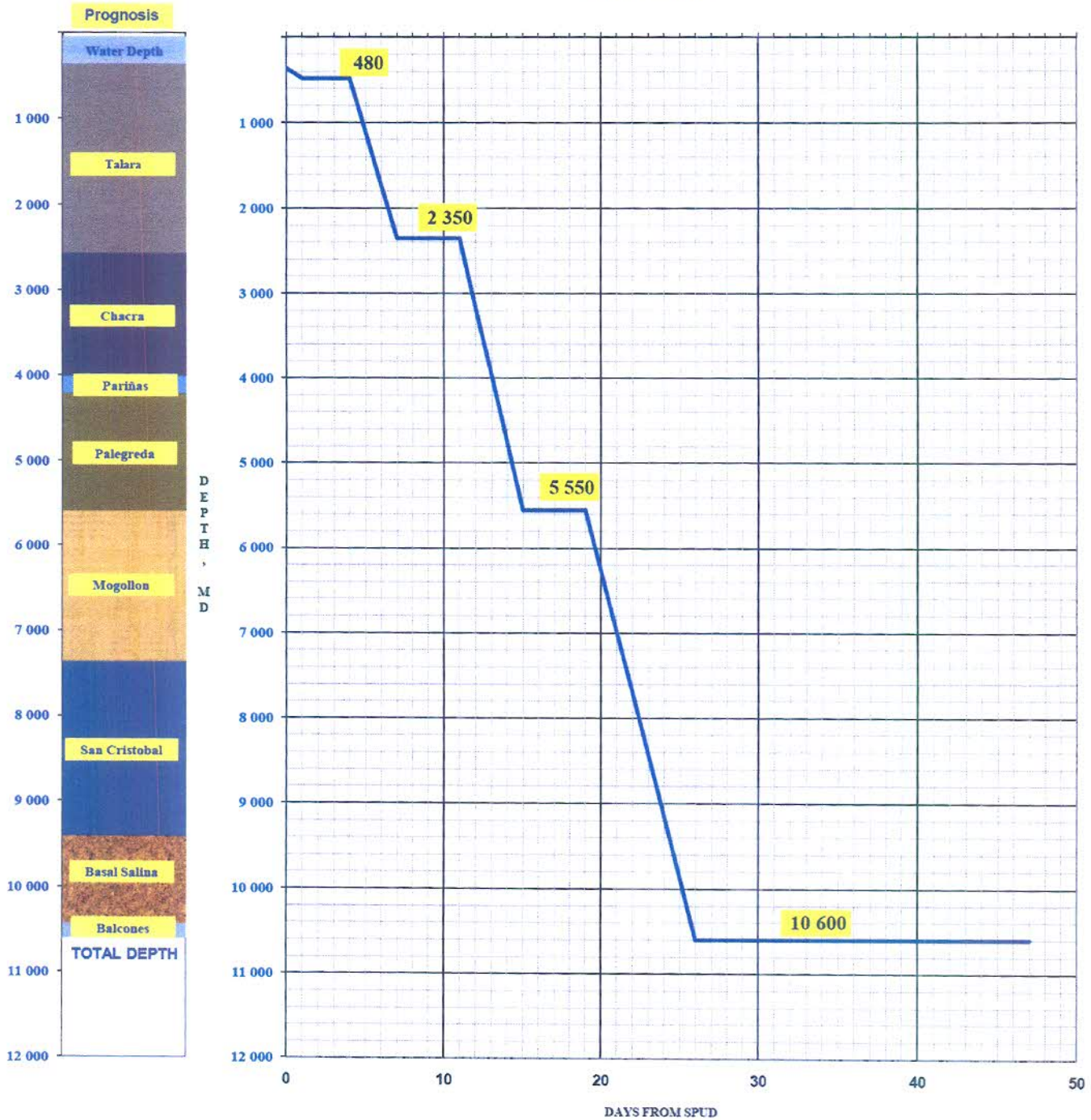
LO16-27D Well Depth Vs. Days
